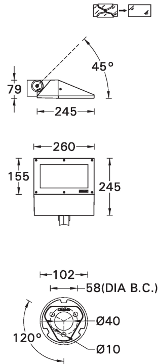
MOUNTING DETAIL
