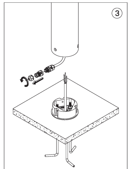
MOUNTING DETAIL
