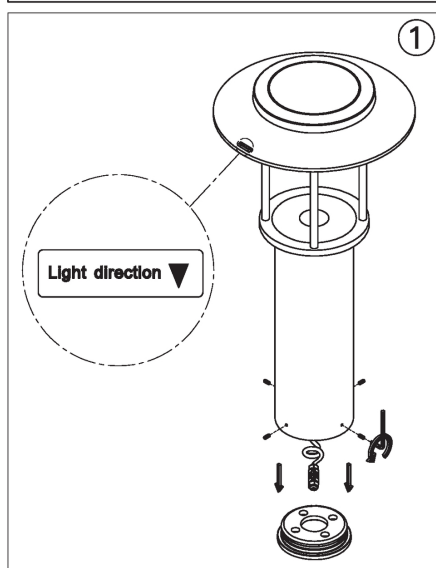
MOUNTING DETAIL
