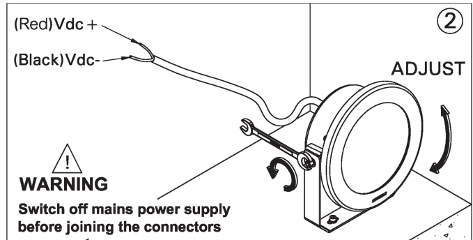
MOUNTING DETAIL
