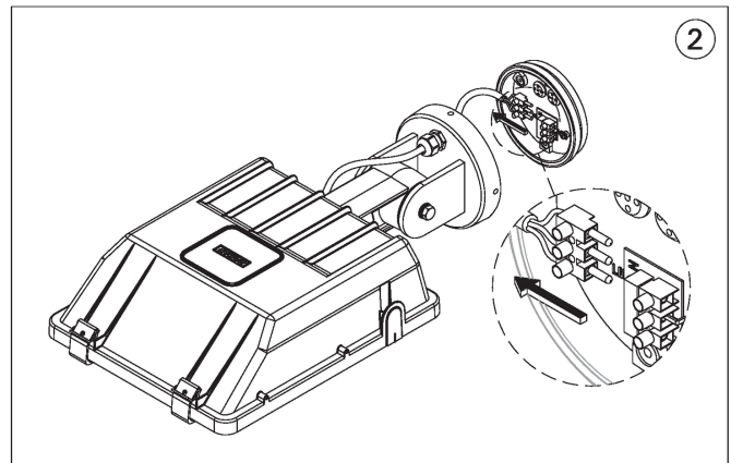
MOUNTING DETAIL
