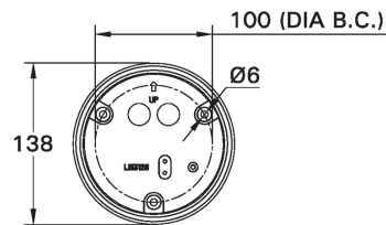
MOUNTING DETAIL
