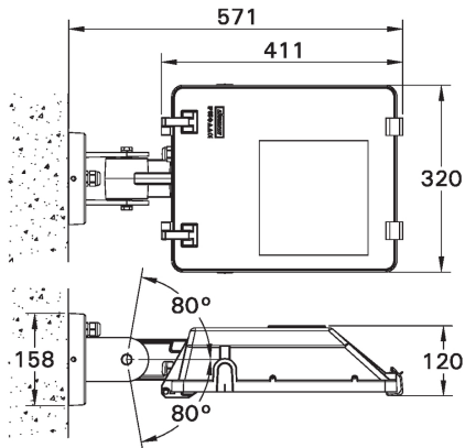
MOUNTING DETAIL
