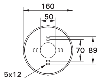
MOUNTING DETAIL
