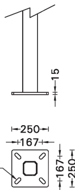
MOUNTING DETAIL
