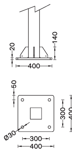
MOUNTING DETAIL
