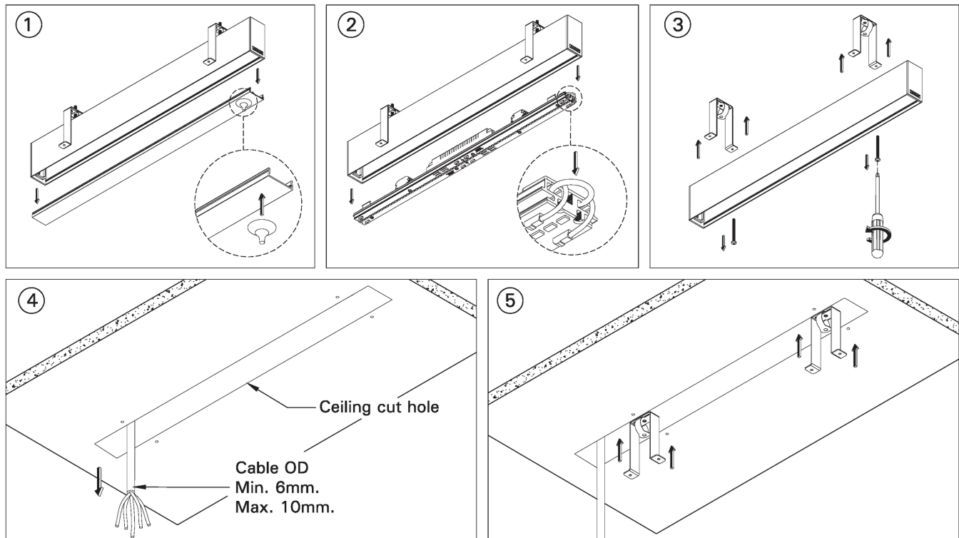
MOUNTING DETAIL
