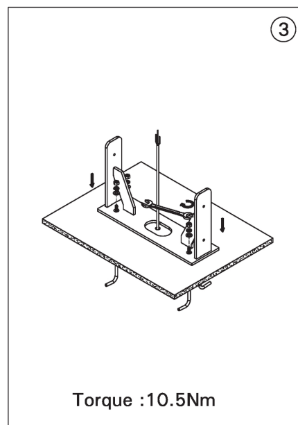
MOUNTING DETAIL
