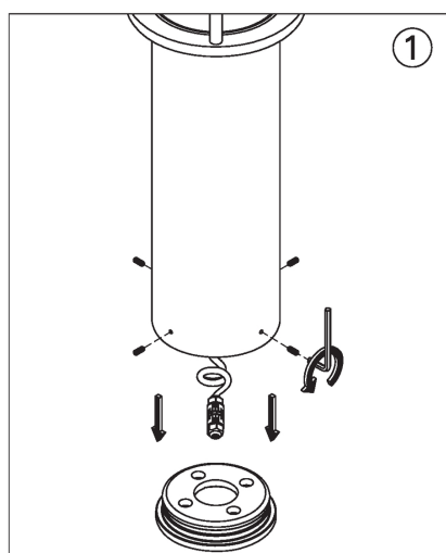
MOUNTING DETAIL
