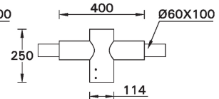
A91160 Double arm mount
