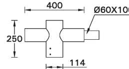
A91060 Single arm mount
