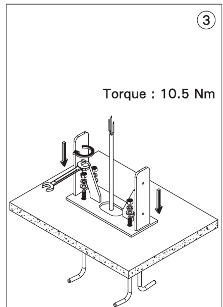
MOUNTING DETAIL
