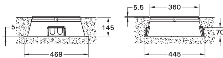
FRONT SURFACE RING KI-60647
