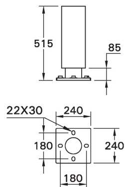
MOUNTING DETAIL
