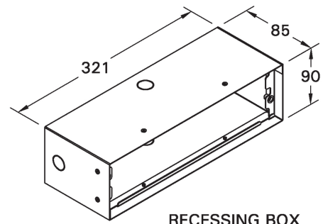
RECESSING BOX
