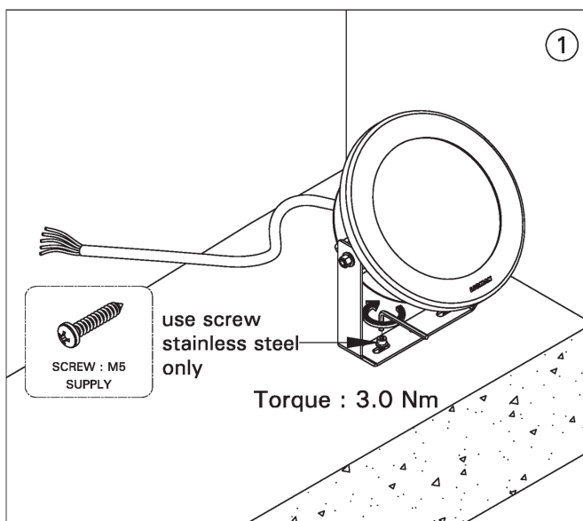
MOUNTING DETAIL
