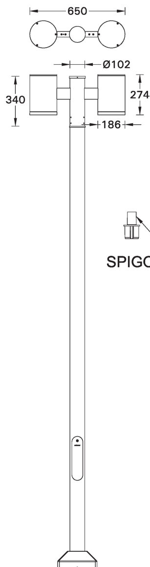
TA-20021, TA-20031 Weight : 9.8 kg Windage Area : 0.43 m 2
