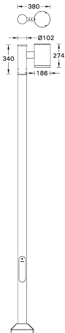
TA-20001, TA-20011 Weight : 5.3 kg Windage Area : 0.37 m 2
