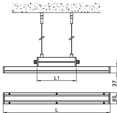
Mounting detail
