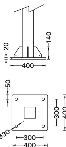
MOUNTING DETAIL
