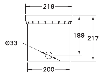
RECESSING BOX IN HDPE
