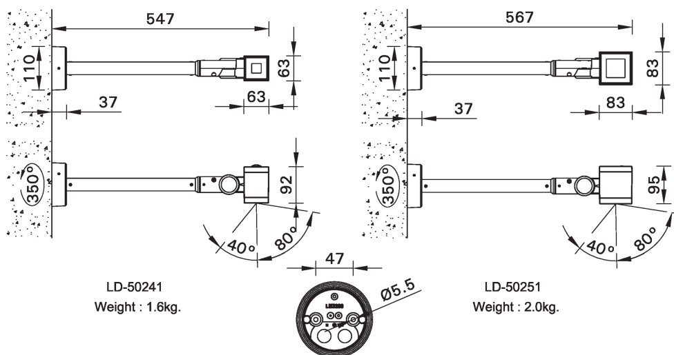
Mounting detail
