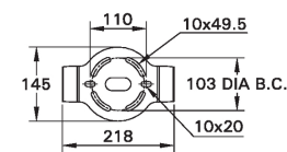
MOUNTING DETAIL QA-50004
