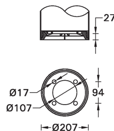
MOUNTING DETAIL
