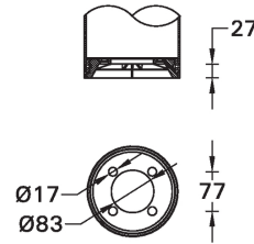
MOUNTING DETAIL
