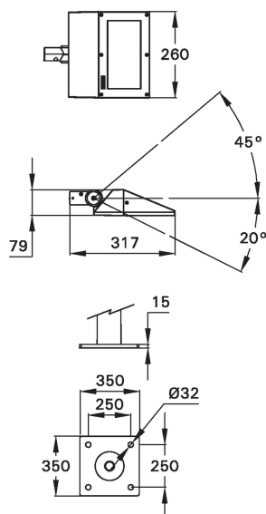
MOUNTING DETAIL
