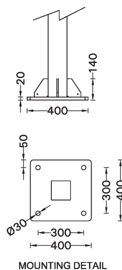
MOUNTING DETAIL
