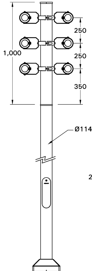
ALUMINIUM POST MOUNTING DETAIL
