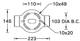
MOUNTING DETAIL
