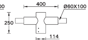
A91160 Double arm mount
