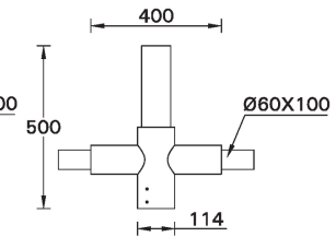
A91360 Double arm mount
