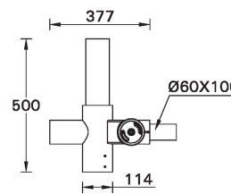
A91660 Single adjustable 50° arm mount
