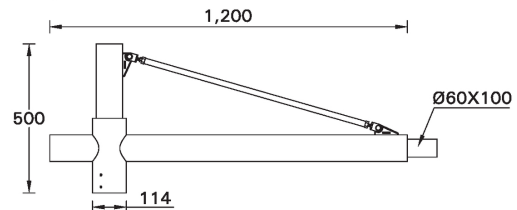
A91460 Single arm mount
