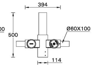
A91760 Double adjustable 50° arm mount
