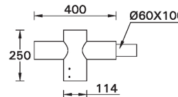
A91060 Single arm mount
