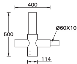
A91260 Single arm mount
