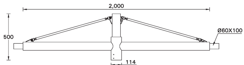
A91560 Double arm mount
