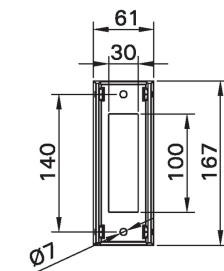
MOUNTING DETAIL
