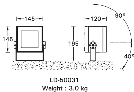
MOUNTING DETAIL
