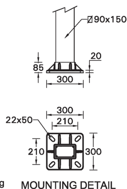
MOUNTING DETAIL
