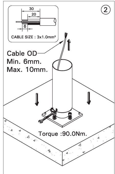
MOUNTING DETAIL
