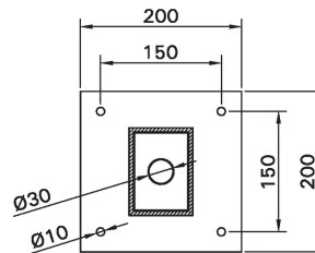
MOUNTING DETAIL
