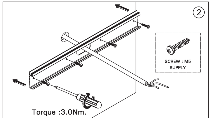
MOUNTING DETAIL
