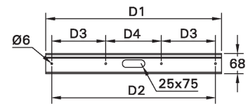
MOUNTING DETAIL
