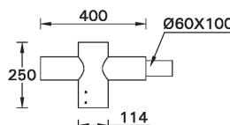
A91060 Single arm mount
