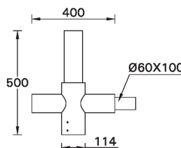
A91260 Single arm mount
