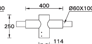
A91160 Double arm mount
