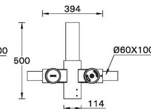
A91760 Double adjustable 50° arm mount
