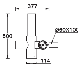
A91660 Single adjustable 50° arm mount
