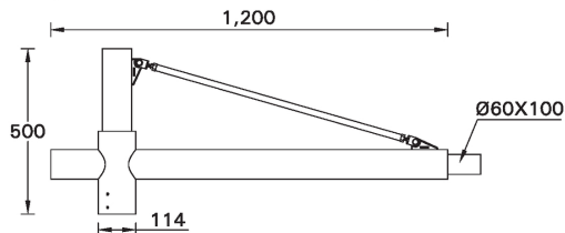
A91460 Single arm mount
