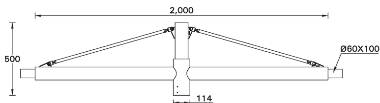
A91560 Double arm mount
