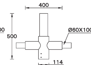
A91360 Double arm mount
