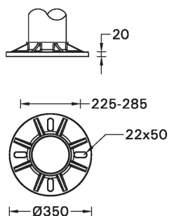
MOUNTING DETAIL
