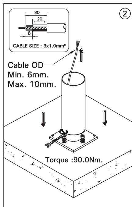
MOUNTING DETAIL
