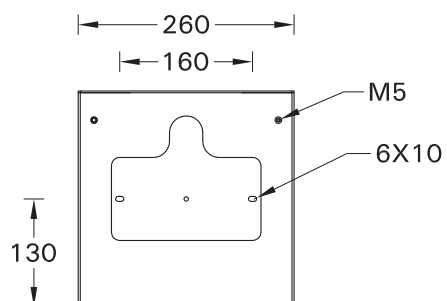
MOUNTING DETAIL
