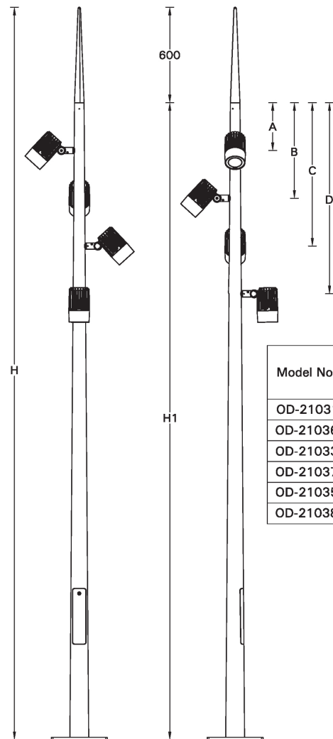
MOUNTING DETAIL
