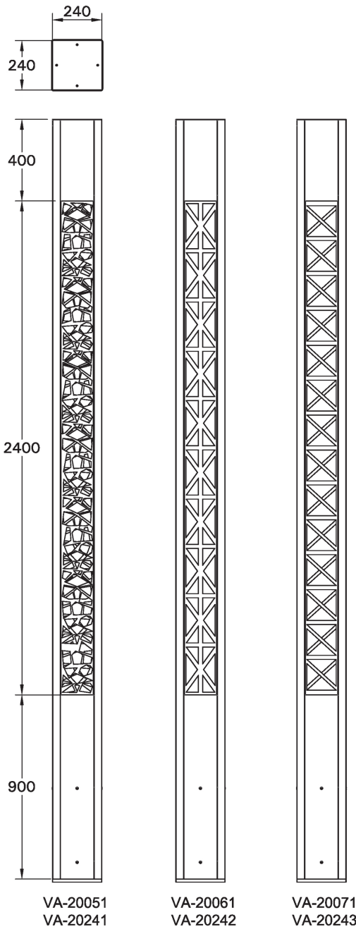
MOUNTING DETAIL
