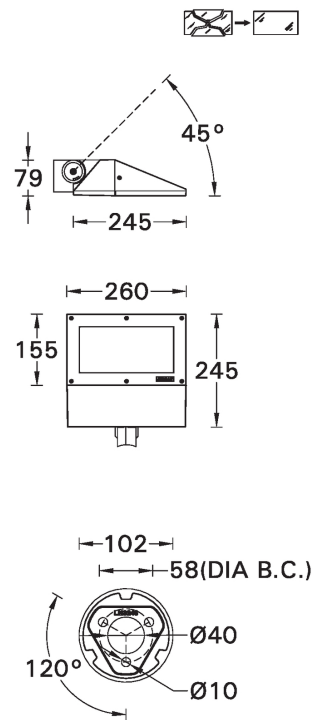
MOUNTING DETAIL
