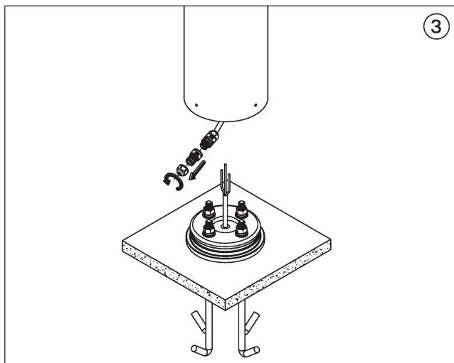
MOUNTING DETAIL
