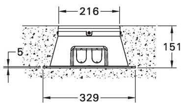
FLAT FRAME KI-60495
