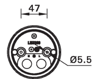
MOUNTING DETAIL
