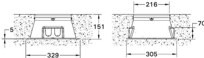
FRONT RECESS RING KI-60475
