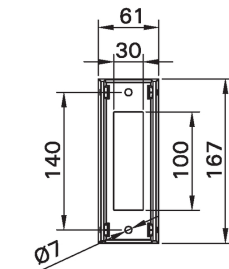
MOUNTING DETAIL
