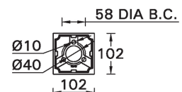
MOUNTING DETAIL
