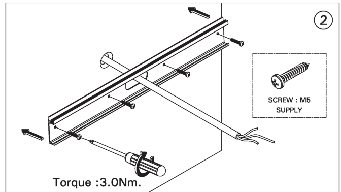
MOUNTING DETAIL
