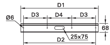
MOUNTING DETAIL
