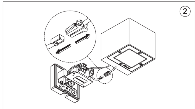
MOUNTING DETAIL
