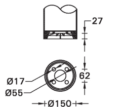
MOUNTING DETAIL
