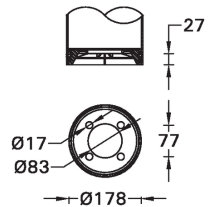
MOUNTING DETAIL
